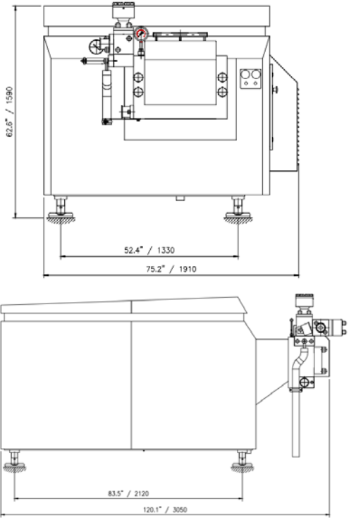
GAULIN 160T
